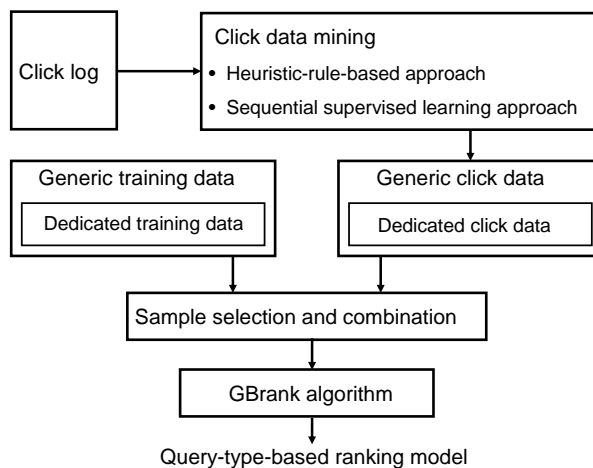
Figure 1: Framework of incorporating click-through data with training data to improve dedicated model for query-type-based ranking.
